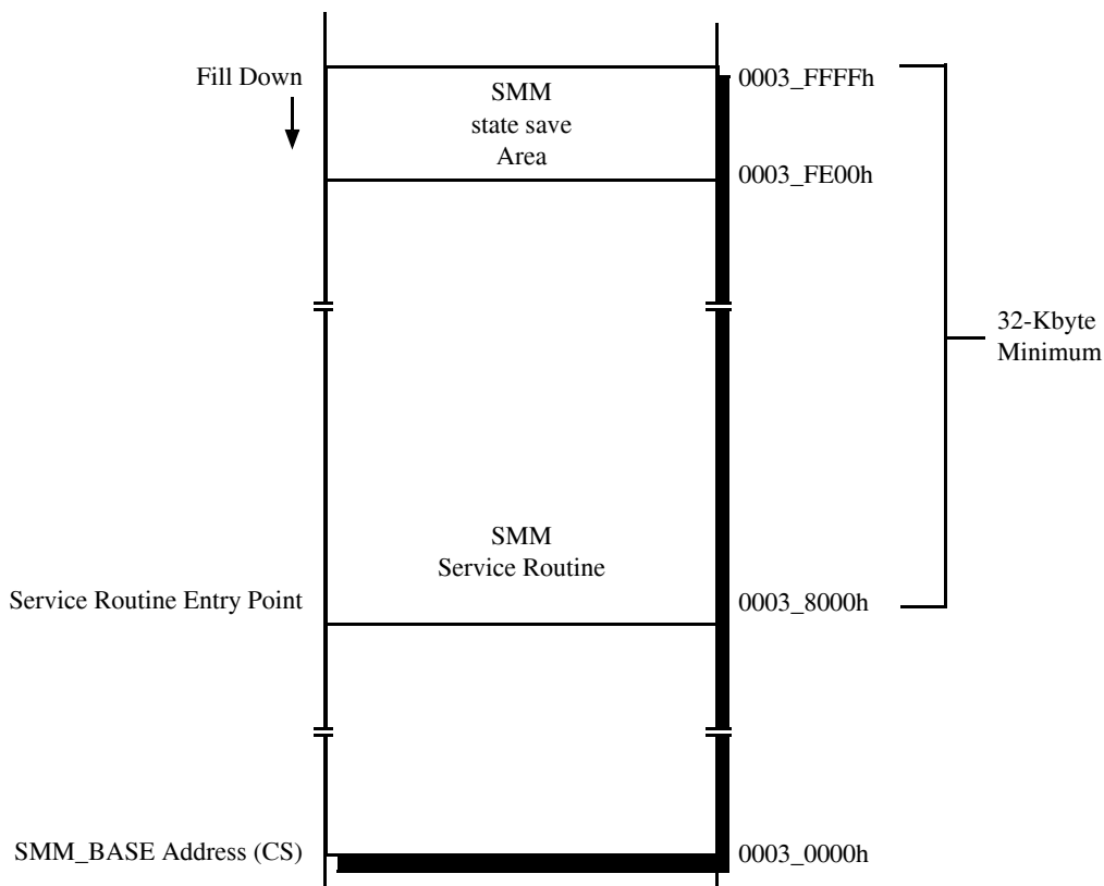
Figure 4. Default SMM Memory Map
